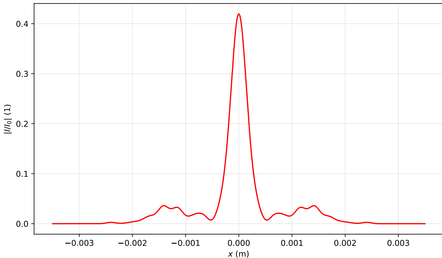
Intensity profile I(x, y = 0, z = 2.866)/I_0 , \text{Pin}=9.0\text{Pcr} , artificial time
